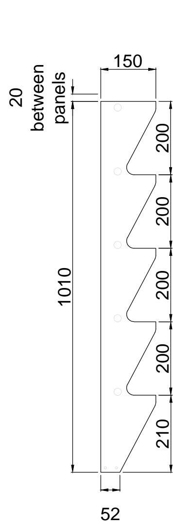
LEFT ELEVATION
