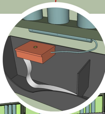
Vegetated screens irrigated with automated system
